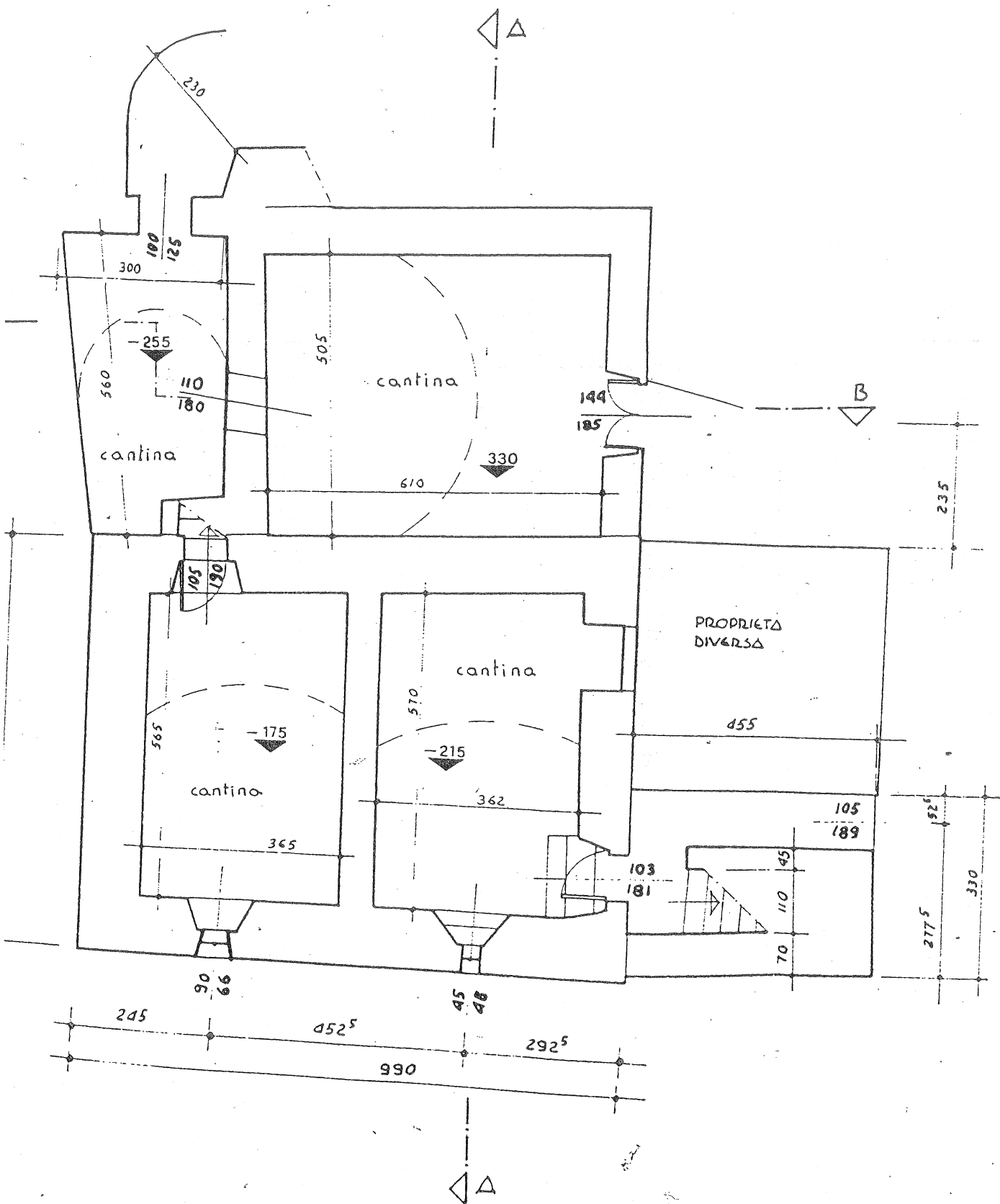
PIANO SEMINTERRATO
